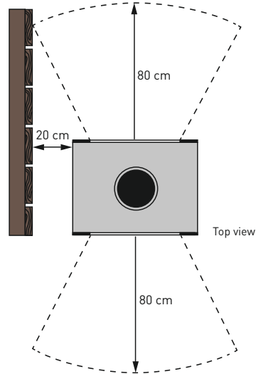
A COMBUSTION CHAMBER WITHOUT LATERAL EXTENSION ELEMENT:
